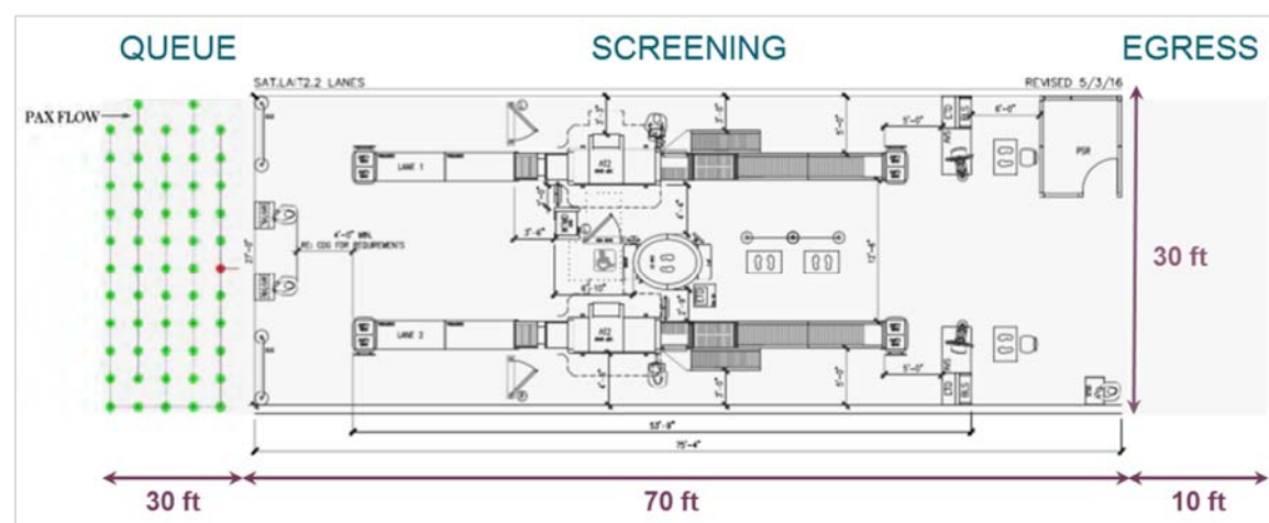
Figure 3-7: Sample Layout for Each Pair of Lanes to Achieve Passenger Throughput with Existing Technology
