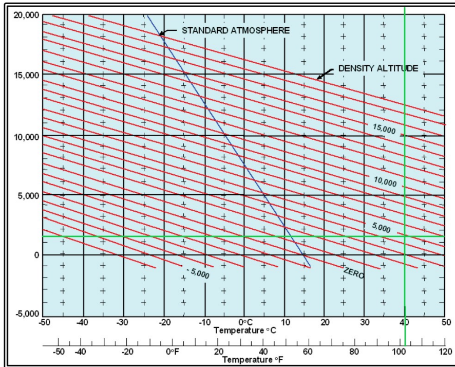
Figure 3-1: Density Altitude for Phoenix-Mesa Gateway Airport Average Maximum Temperature
