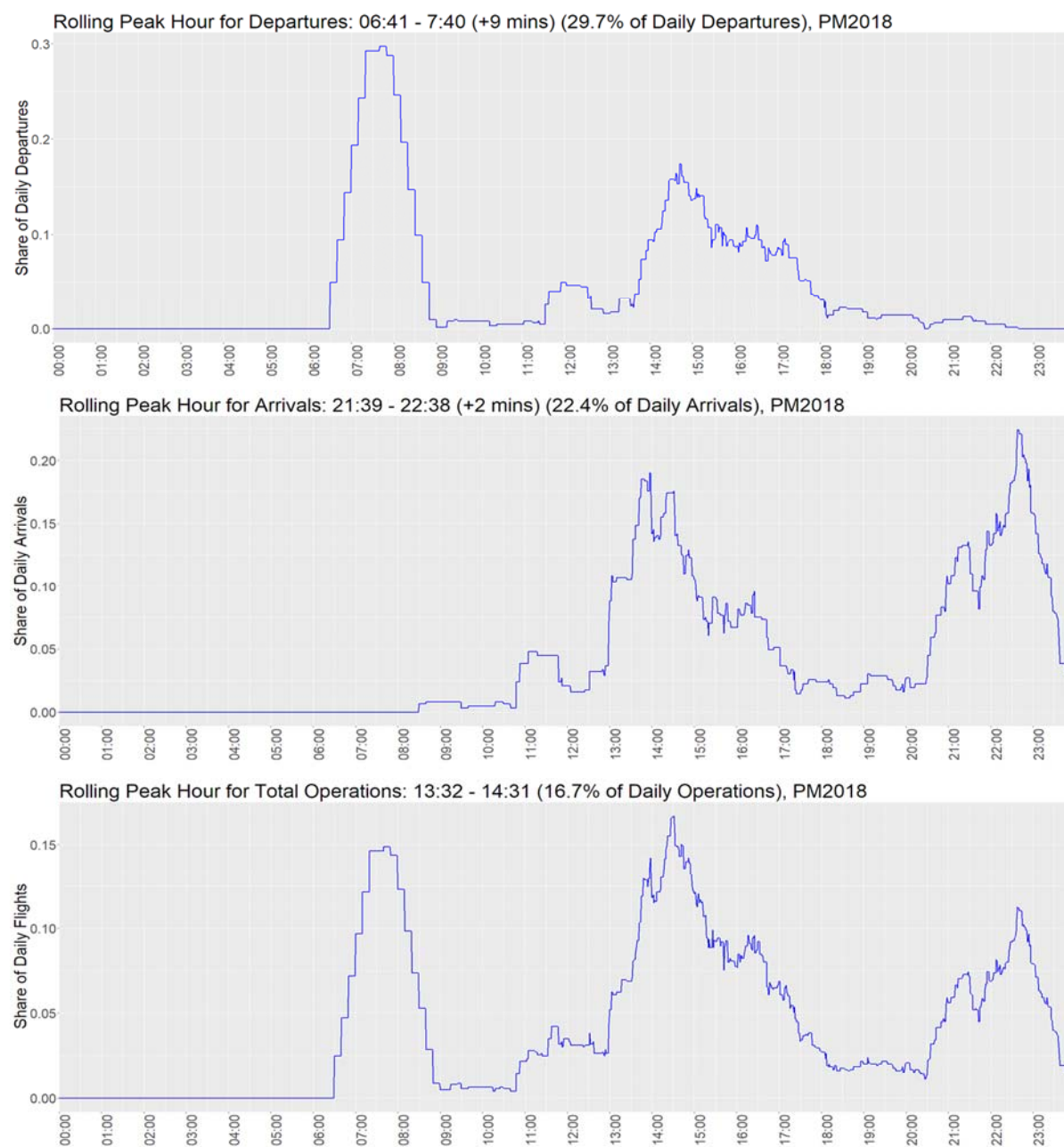
Figure 3-6: Arriving and Departing Flight Activity Profile
